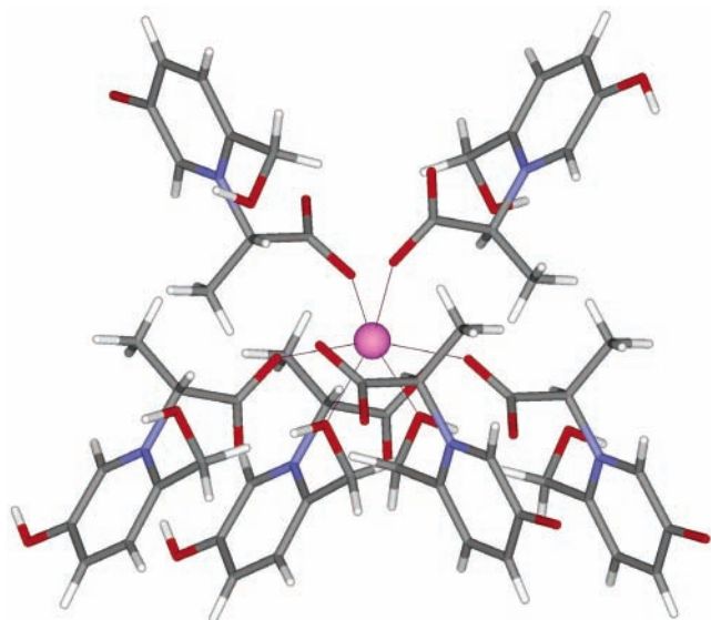
Figure 5. Perspective view of [\text{Na}(\mathbf{1})(\mathbf{1}\text{-H})] crystal structure showing the three phenol and three phenolate forms involved in the distorted octahedral coordination of \text{Na}^+ .
