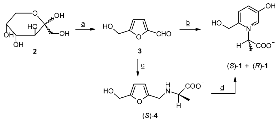
Figure 2. Synthesis of racemic and enantiopure 1: a, Amberlite 15 ( H^+ resin), NEt_3 \cdot HCl , BuOAc/H_2O , reflux under N_2 , 2.5 h, 52% yield; b, 1.0 equiv of L-alanine, 1.9 equiv of 3, EtOH/water (1:1), aq NaOH (32%) \rightarrow pH 9.4, RT (1.5 h) \rightarrow reflux (72 h), 65% yield (sodium salt); c, 1.5 equiv of 3, 2 equiv of L-alanine, water, aq NaOH (32%) \rightarrow pH 8.5, Ni/H_2 , RT, 5 bar, 48 h, 38% yield (ammonium salt); d, 1 equiv of 4 in water, 0 °C, 1.25 equiv of Br_2/MeOH (0.5 h), RT (1 h), 13% yield (ammonium salt). RT, room temperature.
