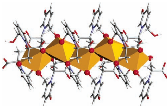
Figure 6. View of the crystal structure of [\text{Na}(\mathbf{1})(\mathbf{1}\text{-H})] showing the one-dimensional \mu_2 -bridging-oxygen polymer with the edge-linked cis -chain of octahedra running along the [100] direction.
