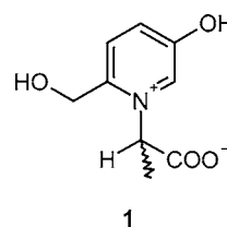
Figure 1. Structure of N -(1-carboxyethyl)-6-(hydroxymethyl)pyridinium-3-ol isolated from a heated aqueous solution of glucose and L-alanine (13).
