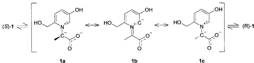
Figure 3. Racemization of 1 in an aqueous alkaline solution under reflux conditions showing the delocalization of the negative charge in the mesomeric forms 1a , 1b , and 1c .
